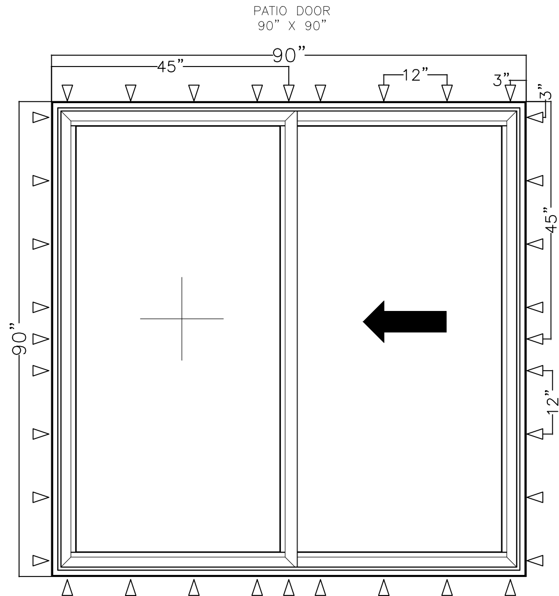
RP 600 XO Sliding Glass Door – FINLESS INSTALLATION MAXIMUM SIZE 90" X 90" DESIGN PRESSURE +/- 25 PSF NON-IMPACT
