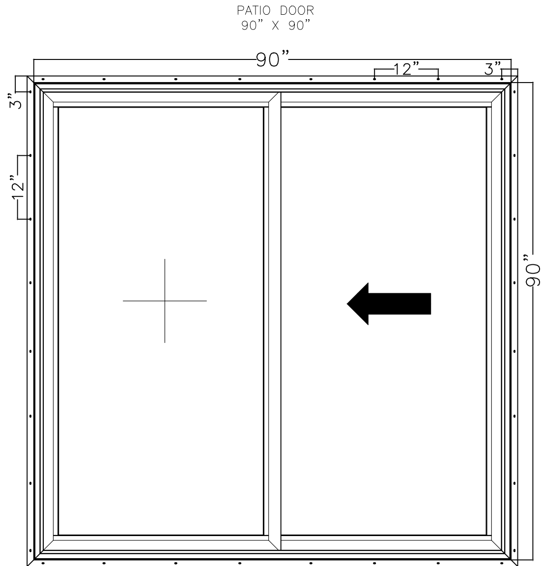
NC 600 XO Sliding Glass Door – FIN INSTALLATION MAXIMUM SIZE 90" X 90" DESIGN PRESSURE +/- 25 PSF NON-IMPACT
