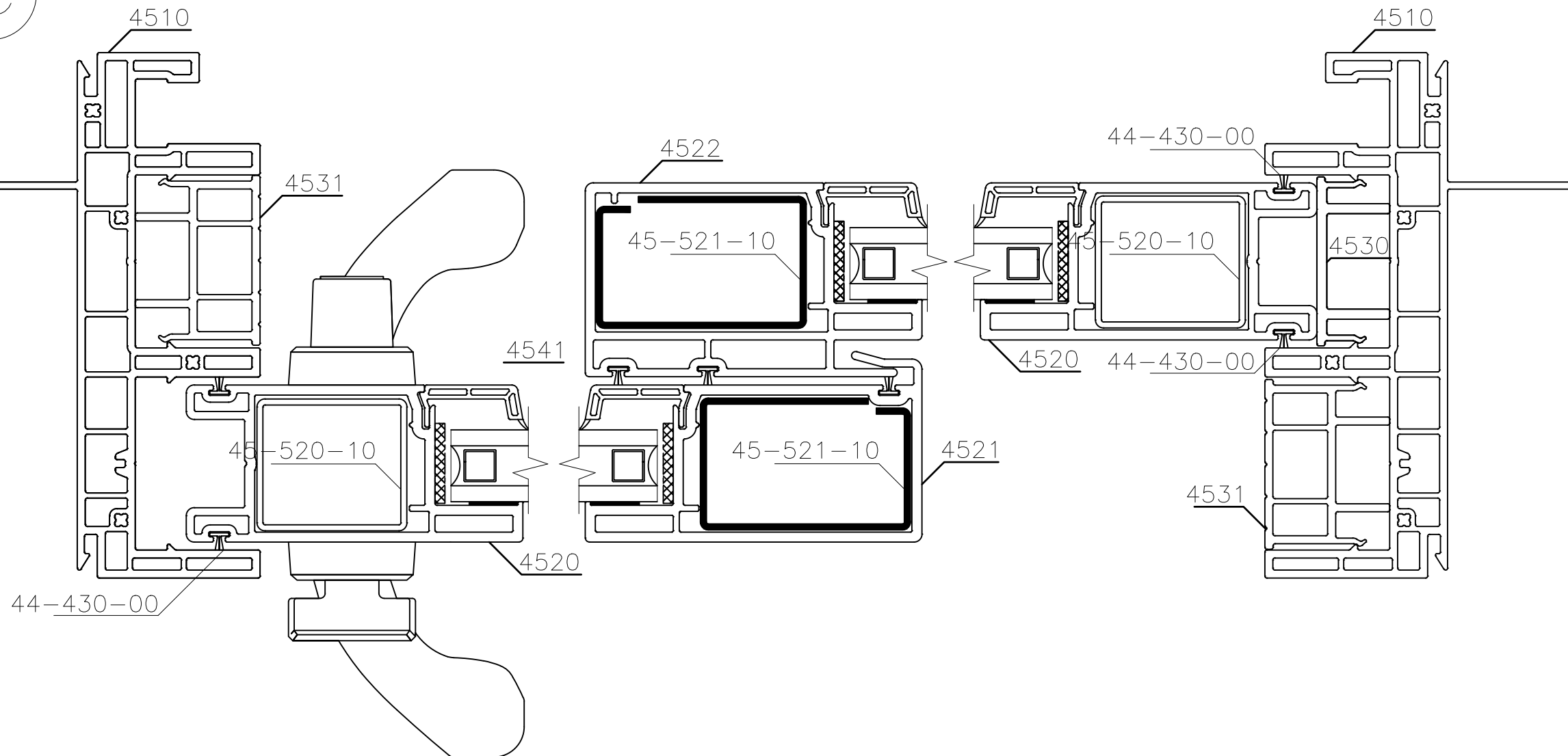
SECTION C-C
